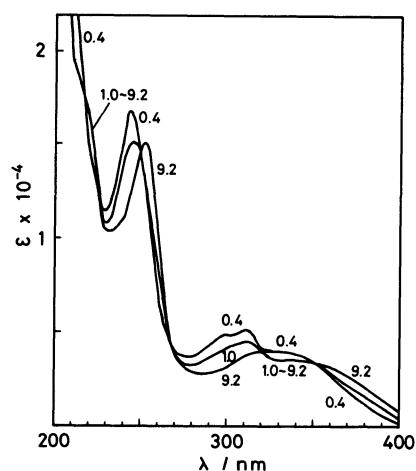
Fig. 2. UV absorption spectra of 3a at various pH values.
