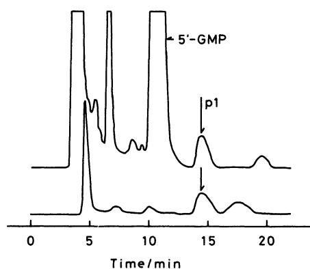
Fig. 1. HPLC chromatograms of 5'-GMP-malonaldehyde reaction mixture. Column: Partisil 10 SAX (4.6φ×250 mm). Upper: UV 254 nm, range 16, 10 μl inj. Lower: FL 365-460 nm, 50 μl inj.
